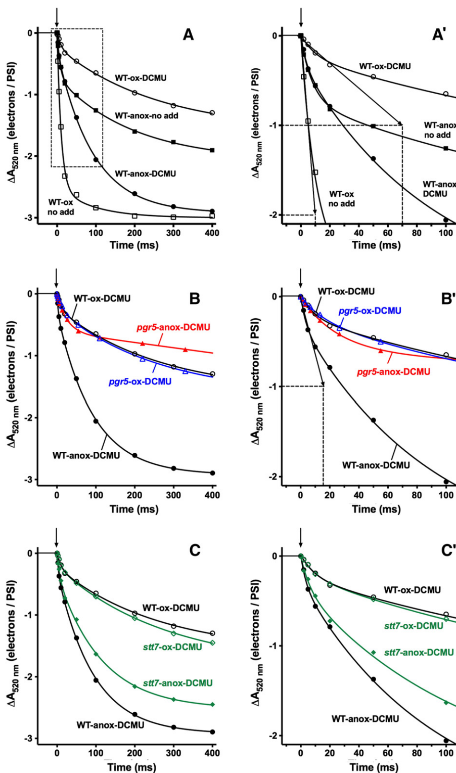
Fig. 4. Decay of the membrane potential upon a light-to-dark transition. For the calibration of the ordinates, the flash-induced absorbance change was measured for each different strain similarly as in Fig. 3 (open circles), so as to normalize the amplitudes obtained in different strains to 1 electron transferred per PSI. After 3 s of illumination, the membrane potential reached a steady-state level (not shown) here shifted to zero for a better comparison of the decay rates. The downward arrow shows when illumination was turned off. Chlamydomonas cells were placed under different conditions oxidic (ox) or anoxic (anox) in the presence or absence of DCMU. For the ease of comparison, the data obtained for the WT, treated with DCMU, are reported identically in all six panels. The kinetics shown here are the result of a single representative experiment. For experimental variations (error bars), please refer to Table 1. The pgr5 strain (B, B') was obtained from [39], and the stt7-9 strain (C, C') from [41].
